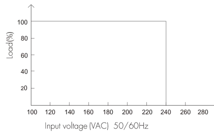
Static characteristic
