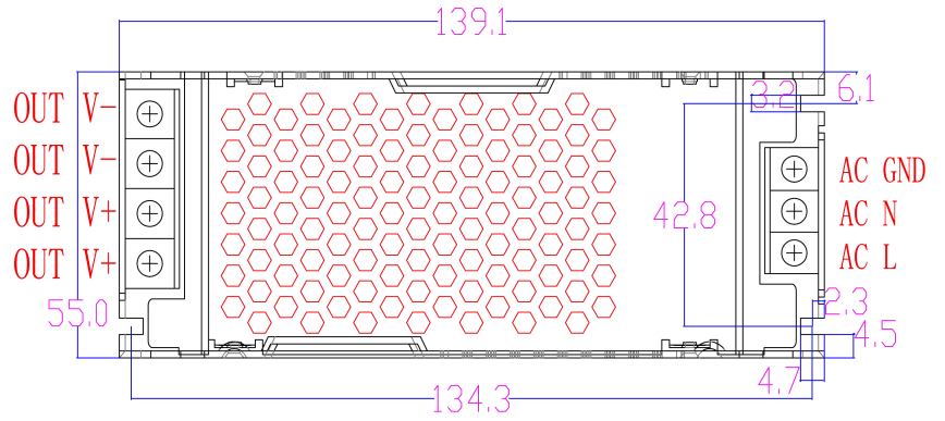
Vertical view
